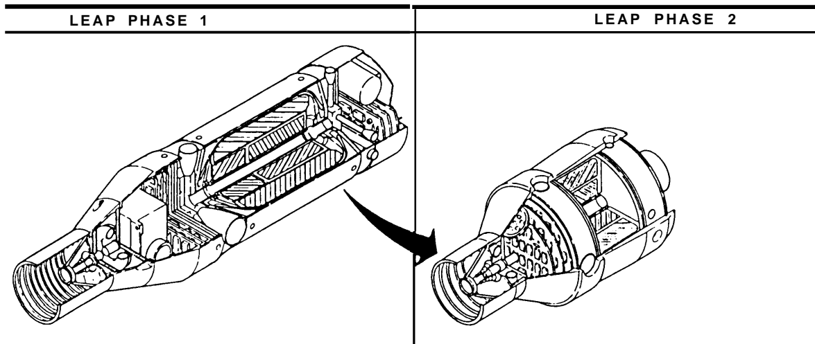
Figure 5-9.— Lightweight Homing Projectile
