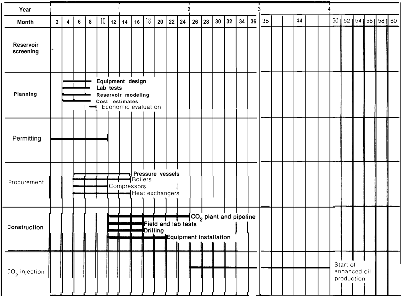
Figure 26.—Schedule for Accelerated EOR CO 2 Flooding Project
