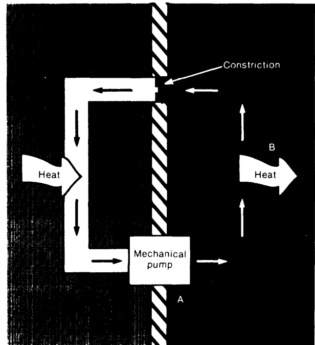
Figure 18.—Principle of an Electric Heat Pump
