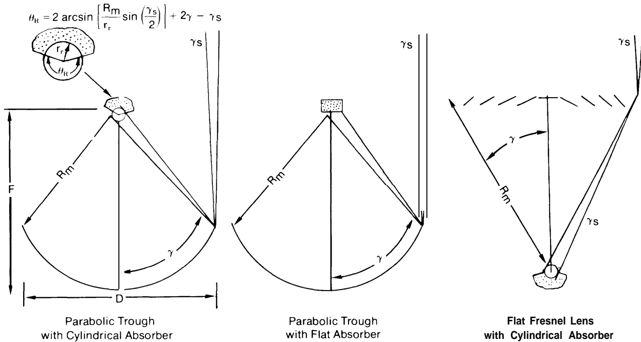
Figure VIII-A-5.—The Solar mane on Three Typical Concentrating Collectors
