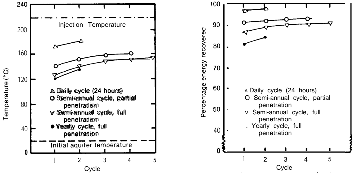
Figure XI-7.— Predicted Performance of an Aquifer Used for Thermal Storage
