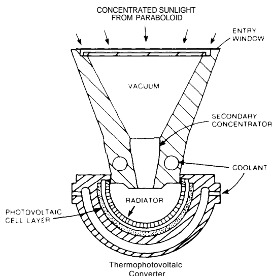
Figure X-5.— Thermophotovoltaic Converter
