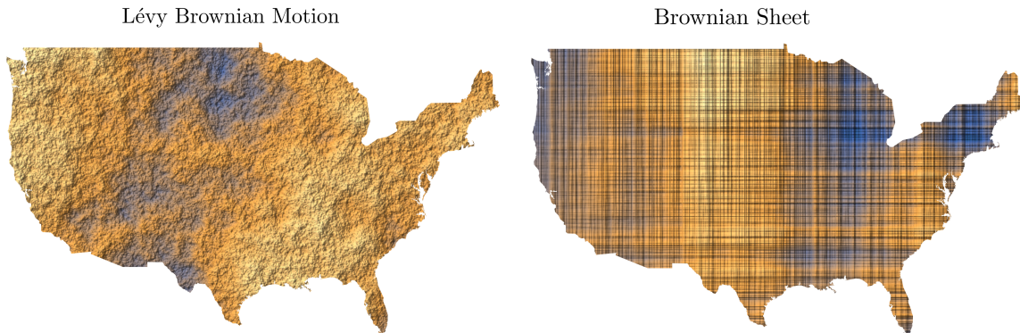
Figure 2. Sample Realizations of Stochastic Processes for d = 2
