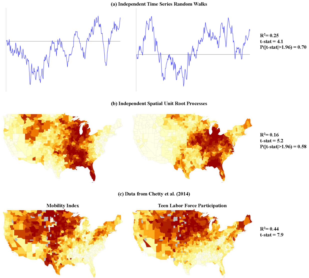
Figure 1. Strongly Dependent Data in Time and Space
